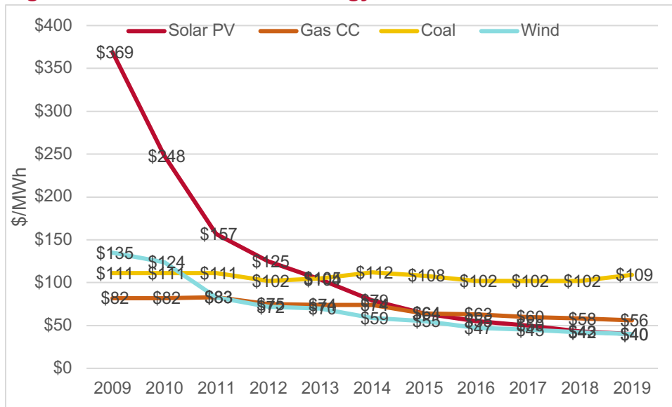
Figure 6. Levelized Cost of Energy, 2009-2018 10
